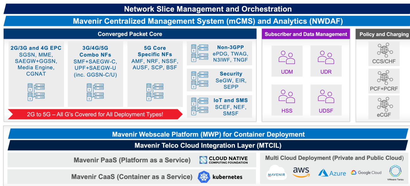
Figure 1: Mavenir Converged Packet Core Solution Components
